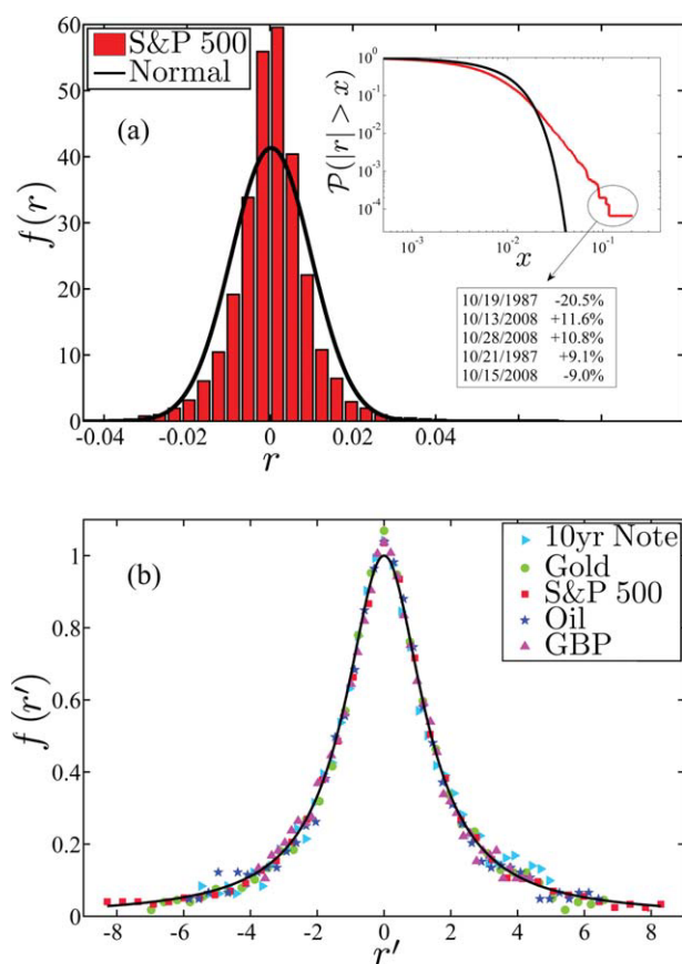
(a) The probability distribution of daily returns for the S&P 500 stock index from January 3, 1950 to November 25, 2009. Inset: Probability that the absolute daily return is above a threshold value, x . The five largest absolute returns are circled and their dates and sizes are shown. (b) The rescaled probability distribution of daily returns for five different traded items: the value of the S&P 500 index, the yield on US 10-year treasury notes, the London Fix AM price of gold, the price of West Texas intermediate oil, and the £/$ exchange rate. The S&P data is the same as used in the previous figure; all other data is from the period January 1985 through May 2010 (except the oil data which begins in January 1986). The black curve is determined as in [21, 22].
